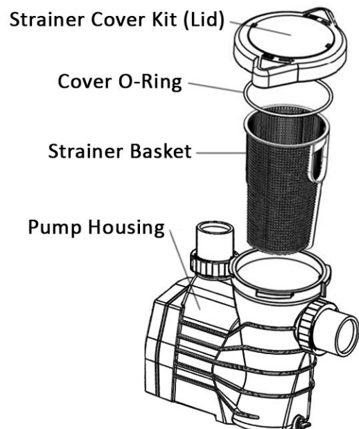
FIGURE 9: Strainer Pot
